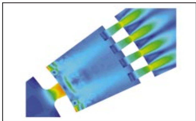
Flow through WhisperFlo trim.
