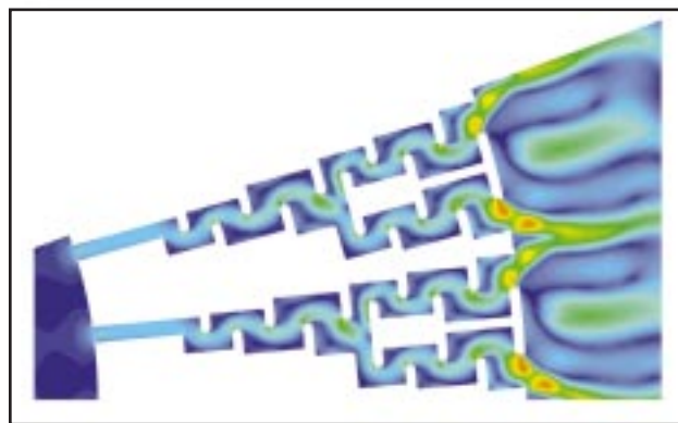
Flow through tortuous path trim.
