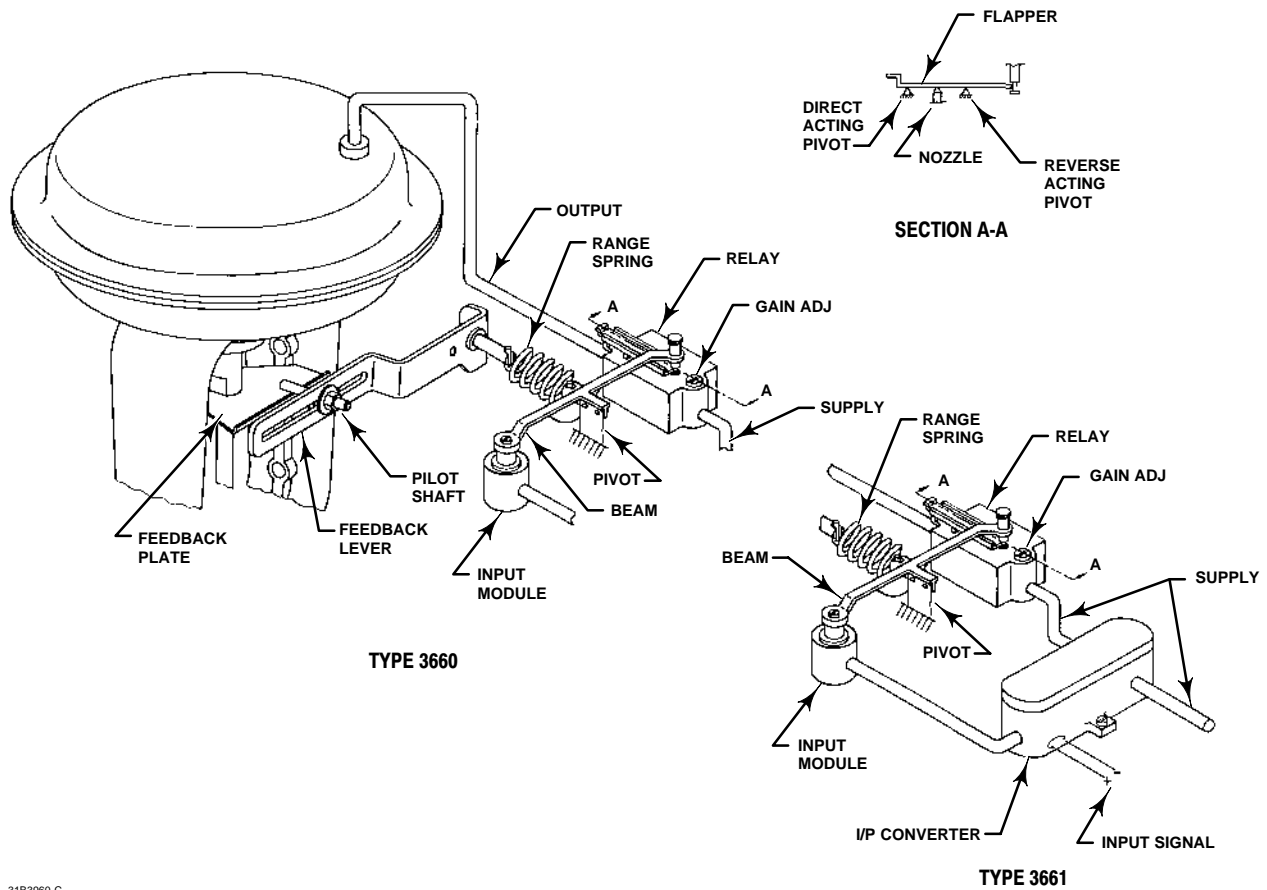
Figure 3. Operational Schematic
