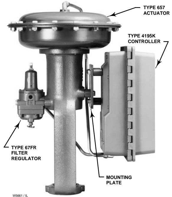
Figure 6. Typical Yoke Mounting
