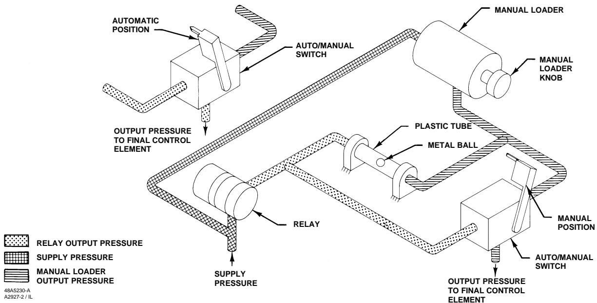
Figure 4. Schematic of Auto/Manual Station
