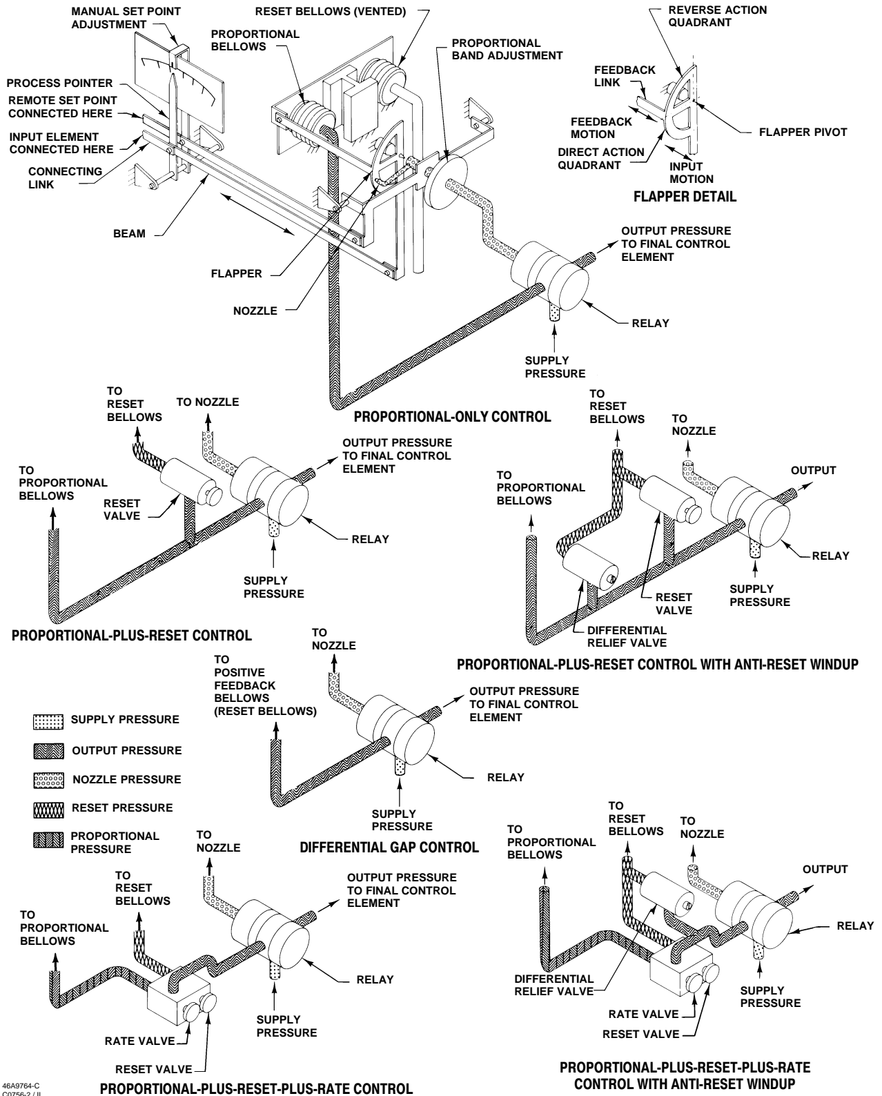
Figure 3. Schematic of 4195K Series Controllers
