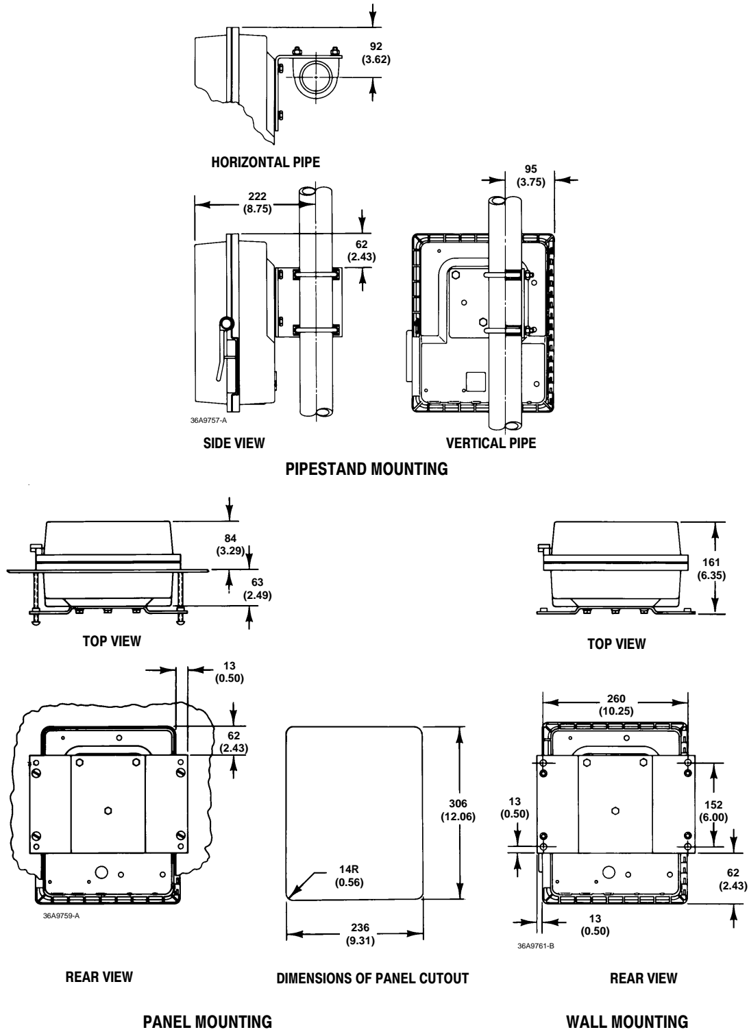
Figure 8. Mounting Dimensions
