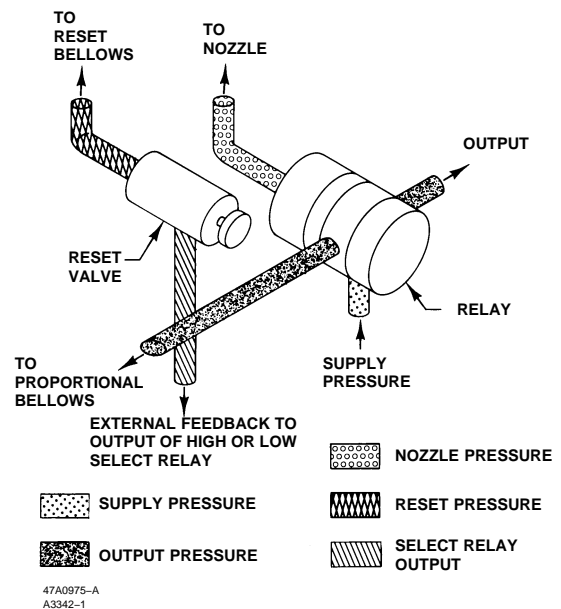
Figure 5. Schematic of External Feedback Option
