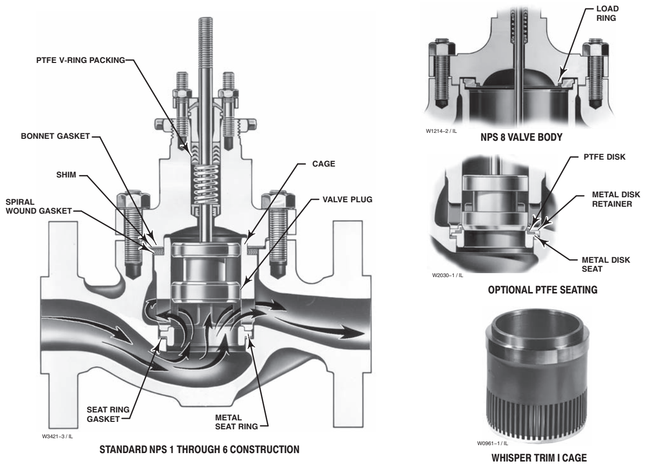
Figure 2. Fisher ES Sectional
