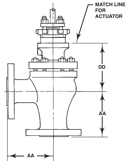
Figure 9. Fisher EAS Dimensions (also see tables 16 and 17)
