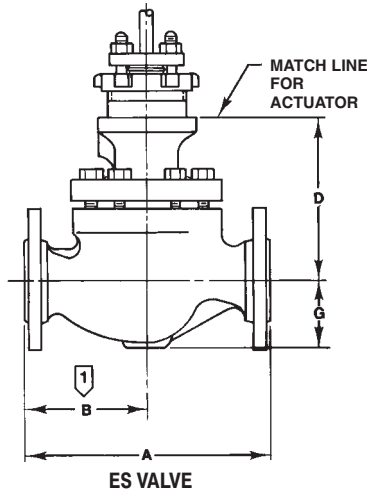
Figure 8. Fisher ES Dimensions (also see tables 13, 14, and 15)
