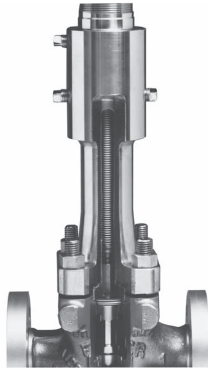
Figure 5. ENVIRO-SEAL Bellows Seal Bonnet
