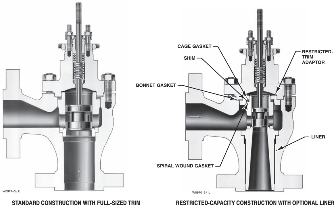
Figure 3. Fisher EAS Sectional
